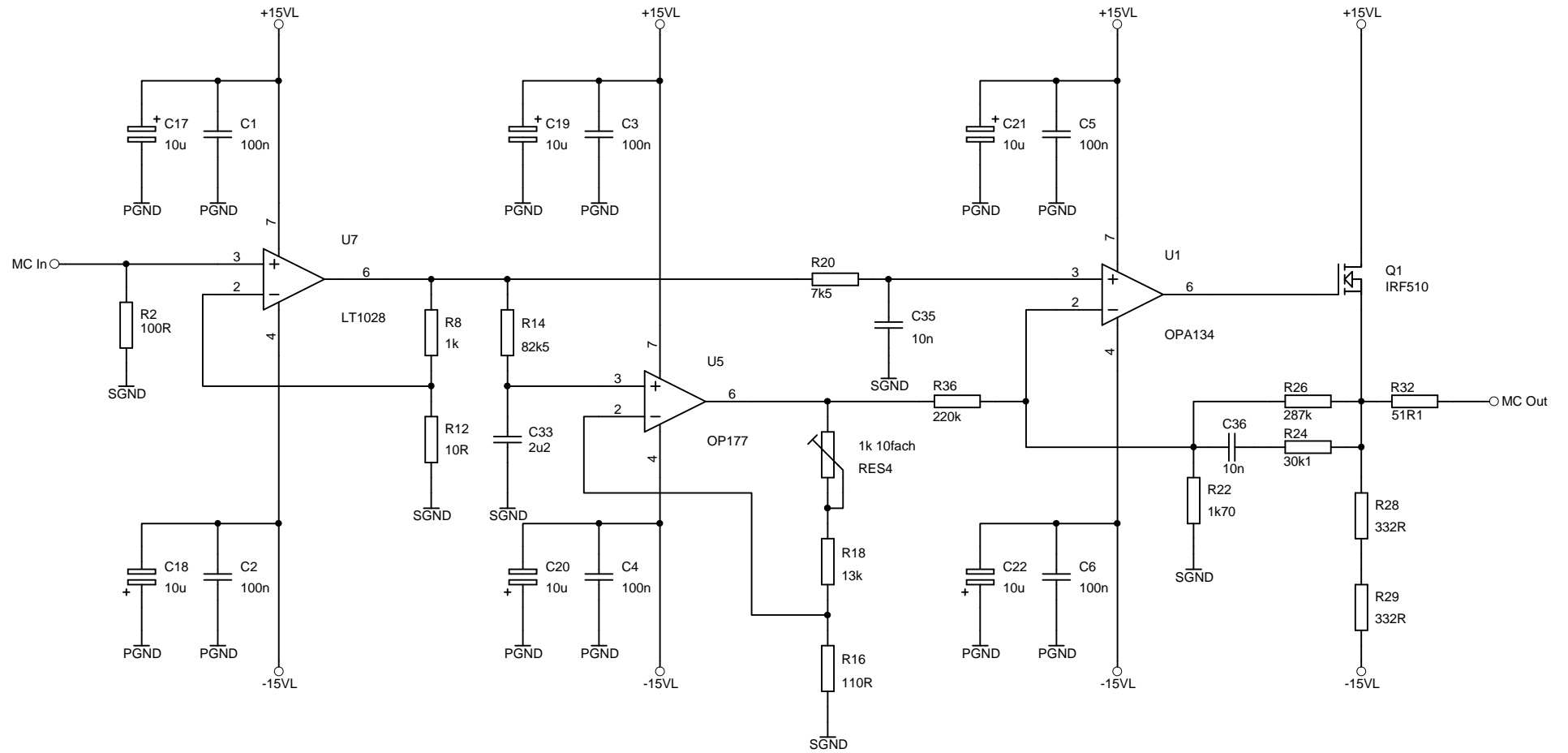
MC PreAmplifier
